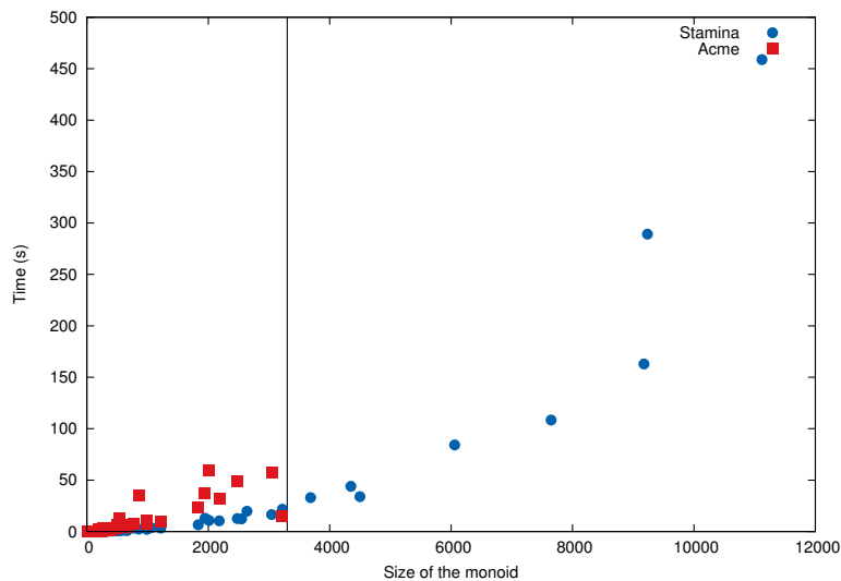
Fig. 1: Random automata of size 10.
